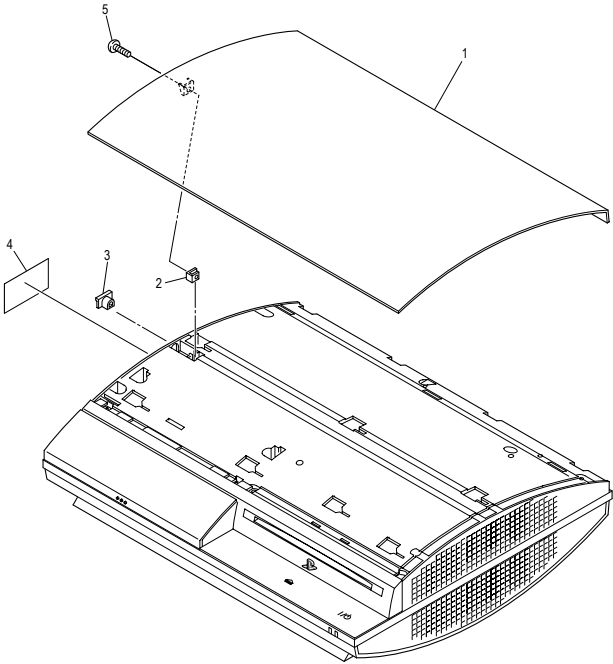
3-1. UPPER PANEL SECTION
