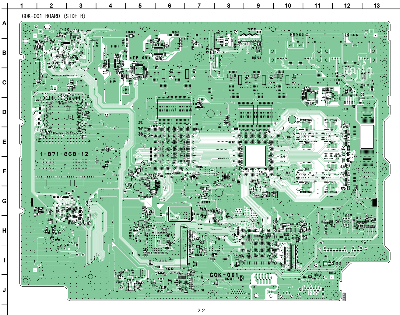
2-2. COK-001 BOARD (SIDE B)
