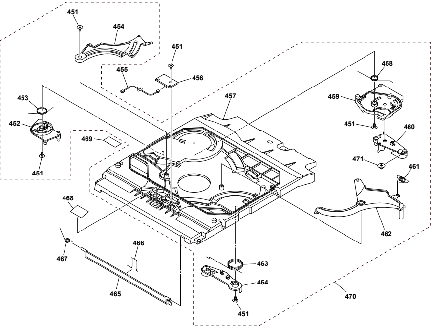
3-10. TOP FRAME COMPLETE ASSY SECTION
