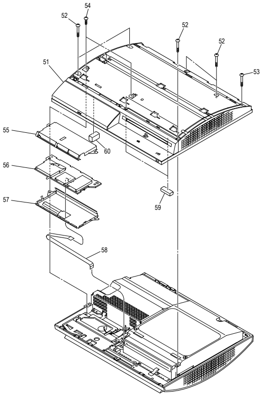
3-2. UPPER CABINET SECTION
