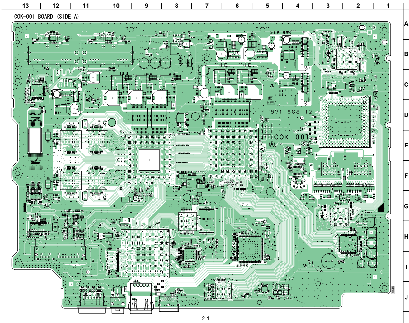
2-1. COK-001 BOARD (SIDE A)
